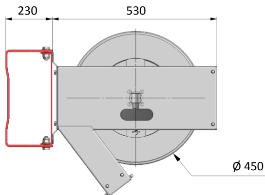
SUPPORT PIVOTANT (OPTION) SWIVEL BRACKET (OPTIONAL)
